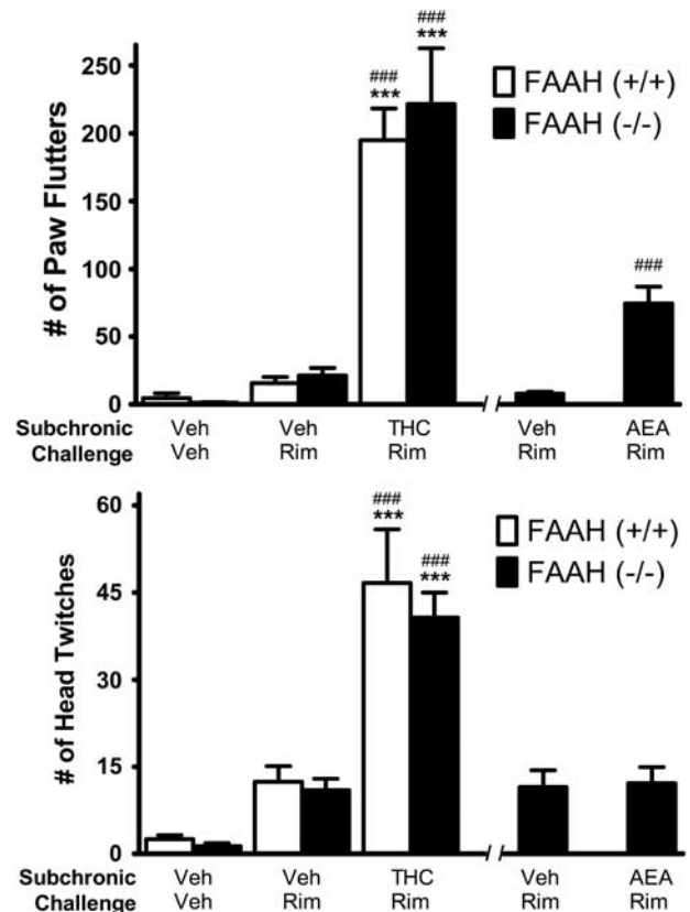
Figure 4 Evaluation of rimonabant (Rim; 10 mg/kg)-precipitated withdrawal in FAAH^{-/-} mice treated subchronically with THC (50 mg/kg twice daily for 5.5 days) or AEA (50 mg/kg twice daily for 5.5 days), and FAAH^{+/+} mice treated subchronically with THC (50 mg/kg twice daily for 5.5 days). Top panel: Rim precipitated significant increases in paw tremors in mice treated repeatedly with THC, regardless of genotype. Rim also precipitated significant increases in paw tremors in FAAH^{-/-} mice treated repeatedly with AEA, though the magnitude of this effect was considerably less than in mice treated repeatedly with THC. Bottom panel: Rim precipitated significant increases in head twiches in mice treated repeatedly with THC, regardless of genotype. Rim did not elicit any differences in head twiches between FAAH^{-/-} mice treated subchronically with vehicle or AEA. *** p < 0.001 vs corresponding subchronic vehicle-vehicle-challenge group of the same genotype. ### p < 0.001 vs corresponding subchronic vehicle-rimonabant challenge group of the same genotype. Data are presented as mean \pm SEM; n = 6 mice/condition.
