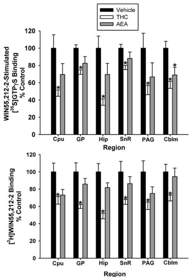
Figure 9 Subchronic THC attenuates CB _1 receptor binding and G-protein activity, whereas subchronic AEA produces minimal CB _1 receptor adaptation. Net WIN55,212-2-stimulated [ ^{35}\text{S} ]GTP \gamma S binding (top) and [ ^3\text{H} ]WIN55,212-2 binding (bottom) in THC- and AEA-treated FAAH ^{-/-} mice are expressed as a percentage of control (vehicle-treated) mice ( n = 8–12 mice/group, * p < 0.05 different from vehicle-treated group by one-way ANOVA with a post hoc Dunnett's test).
