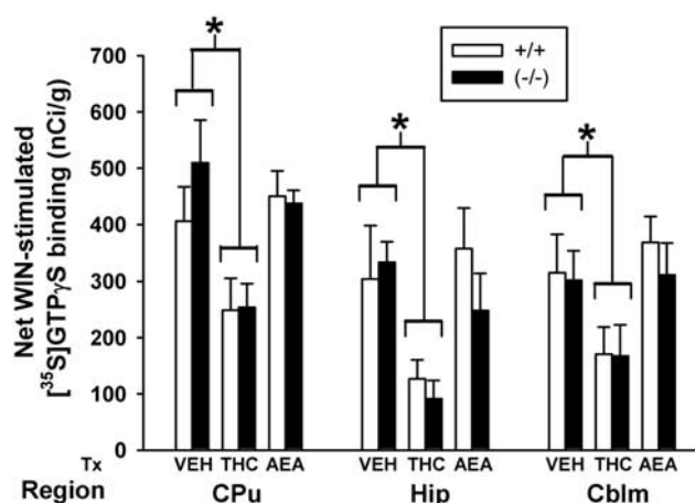
Figure 5 Subchronic THC reduces CB 1 receptor-mediated G-protein activity in both FAAH +/+ and FAAH -/- mice, but subchronic AEA does not significantly alter CB 1 receptor-mediated activity. Densitometric analysis of net WIN55,212-2-stimulated [ 35 S]GTPγS binding in FAAH +/+ and FAAH -/- mice treated with vehicle (VEH), THC, or anandamide (AEA) in CB 1 receptor-containing brain regions: caudate-putamen (CPU), hippocampus (Hip), and cerebellum (Cblm). No significant genotype differences were observed regardless of treatment or brain region. Values represent mean net [ 35 S]GTPγS binding (nCi/g) ± SEM, n = 4–6 mice/group (* P < 0.05 by two way ANOVA with post hoc Dunnett's test).
